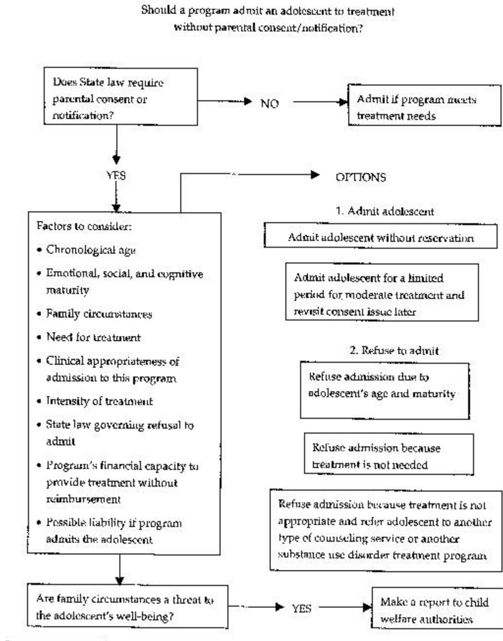
Figure 8-1: Decision Tree
